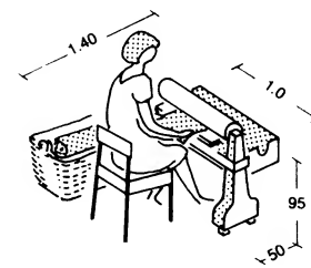
13 Electrical clothes press
